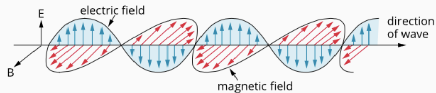
7.3.2 • The electric and magnetic fields in electromagnetic radiation are perpendicular to each other and are both perpendicular to the direction of propagation of the radiation.
