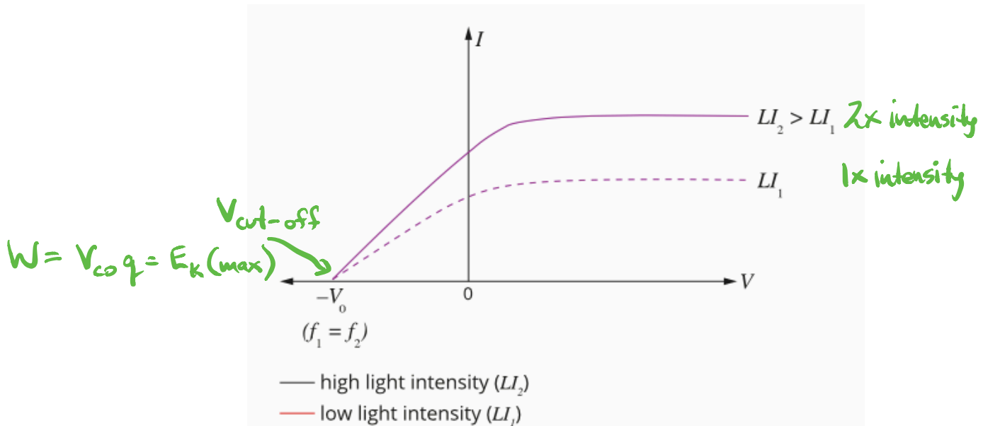
7.4.9 • Photoelectric current ( I ) plotted as a function of the voltage ( V ) applied between the cathode and the anode in the photocell for different light intensities. For brighter light of the same frequency, there is a higher photoelectric current, but the same stopping voltage.
