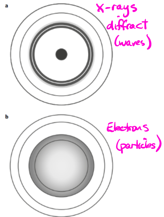
FIGURE 7.6.8 These diffraction patterns were taken by using (a) X-rays and (b) a beam of electrons with the same target crystal. Their similarity suggests a wave-like behaviour for the electrons and an electron de Broglie wavelength similar to that of X-rays.
