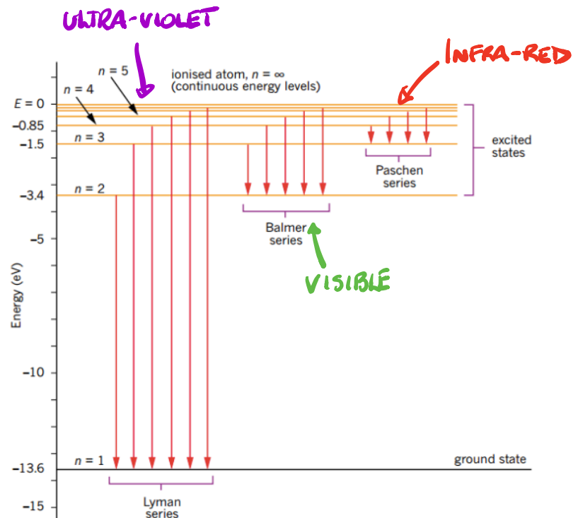
FIGURE 7.5.6 An energy level diagram for hydrogen. An electron in the ground state ( n=1 ) has an energy of (-)13.6 eV. For higher energy levels ( n > 1 ), the energy levels can be seen to crowd together.
